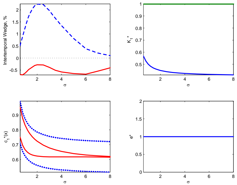
Figure 2: Benchmark parameterization
