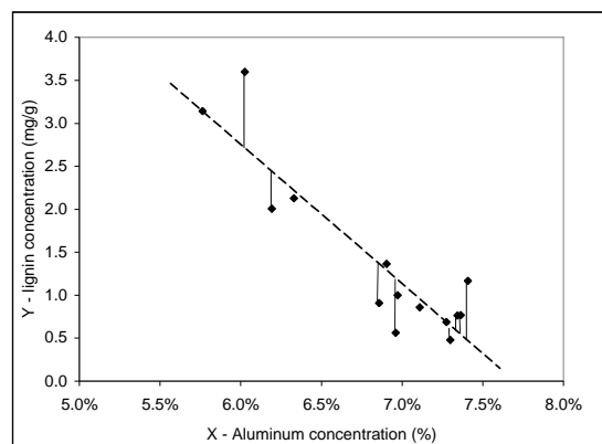
Fig. 5. Lignin concentrations (natural organic matter exclusive to vascular plants) vs. aluminum concentrations in lake sediments.
