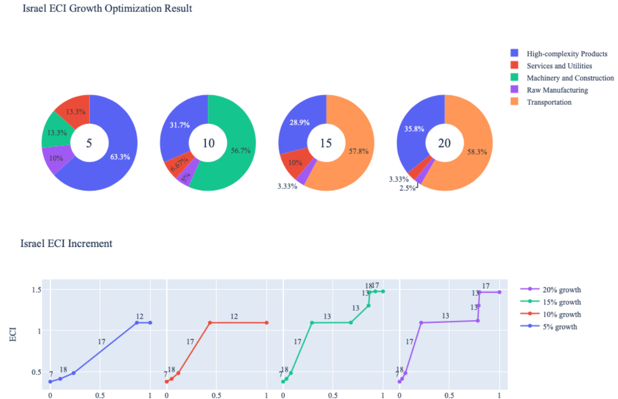
Figure 6: Greedy Based ECI Improvement Results of Israel in 2018 with Different Budgets
