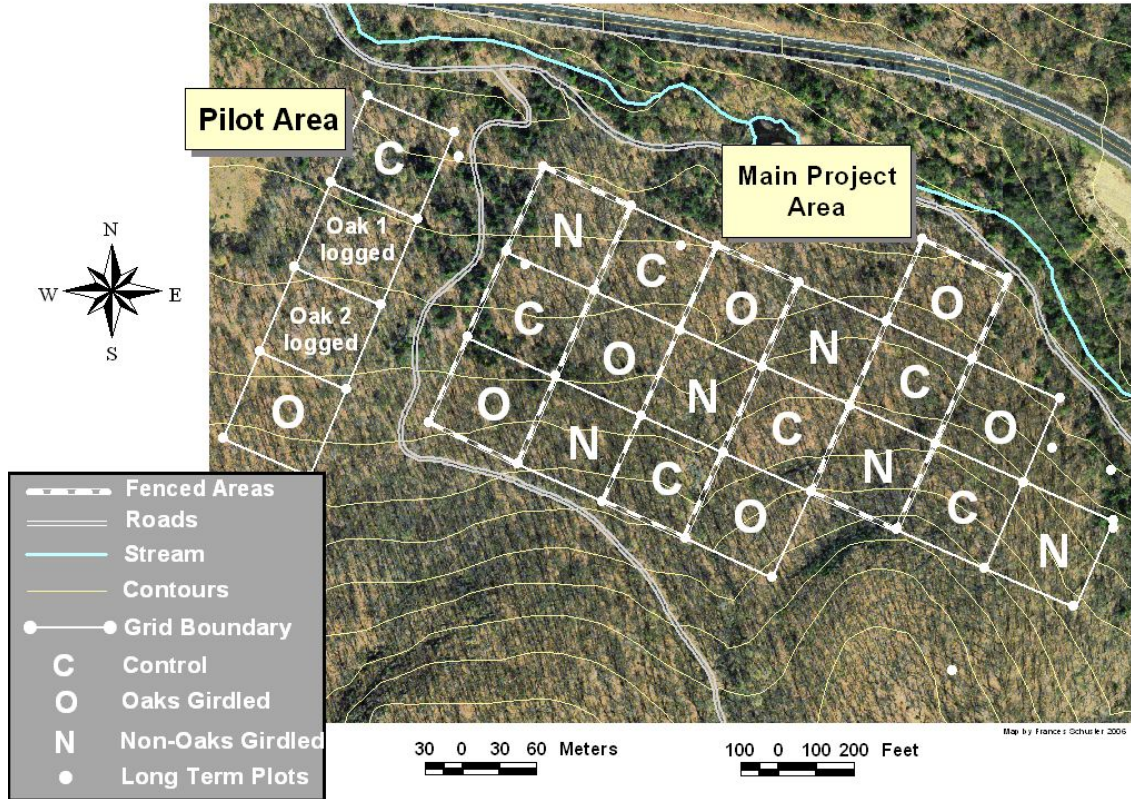
Figure 2. The study site at Black Rock Forest, Orange County, NY. Grid boundaries indicate the limits of twenty 5,625 m 2 plots, inside each of which the 625 m 2 plots are centered. Contours indicate 10 m increments in elevation, from 140 m at the base of the slope (top of photo). Letters indicate planned canopy removal treatments. Map courtesy of Frances Schuster, Black Rock Forest.
