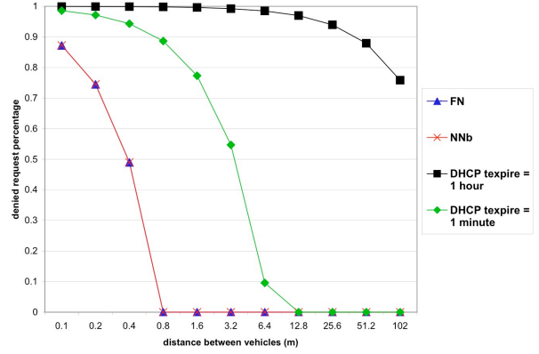
Figure 11: Denied request fraction is the percentage of DHCP requests an AP cannot serve. Due to the length of DHCP leases, a DHCP pool can become saturated very quickly. With IP Passing, only the minimum amount of IPs required to satisfy all vehicles passing through the AP coverage area will be used.
