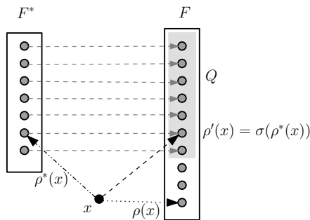
Figure 3: Figure showing maps \rho : S \rightarrow F , optimal map \rho^* : S \rightarrow F^* applied to point x \in S , and also the matching F^* \rightarrow F .
