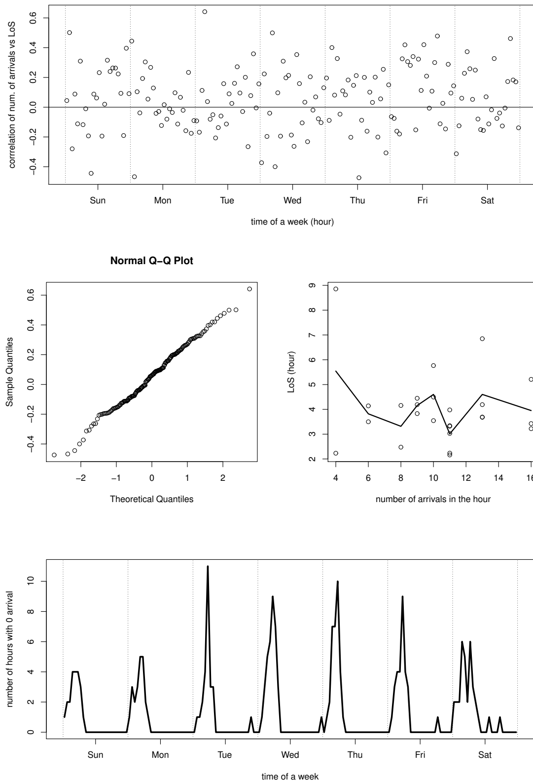
Figure 3 Top: the estimated linear correlation between the number of arrivals and the mean LoS for each hour of a week; Middle left: the Q-Q (quantile) plot of the correlation coefficients compared to a Gaussian distribution; Middle right: an example of the relationship between the number of arrivals and the mean LoS at noon on Monday, while the solid line is the average for each column of points; Bottom: the number of hours with no arrival for each hour in a week.
