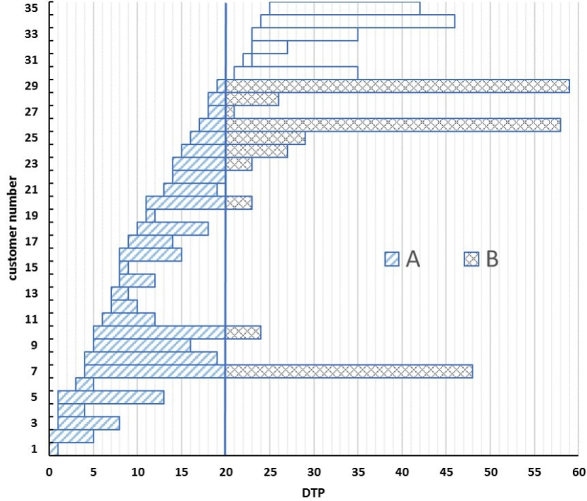
Figure 2 An example of a periodic queueing system with d = 5 and n = 4 . The vertical line is placed at time nd = 20 . Area A corresponds to C_Q(4) in (18) below, while Area A \cup B corresponds to C_L(4) in (18).
