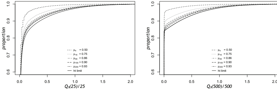
FIGURE 2: Display of the empirical cdf of Q_n(t)/t for 0 \leq t \leq T in the \sum P_i/D/1 queue with Q_n(t) in (22), \beta = \gamma = \mu = 1 for T = 25 (left) and 500 (right), compared to Q(t)/t in (32).
