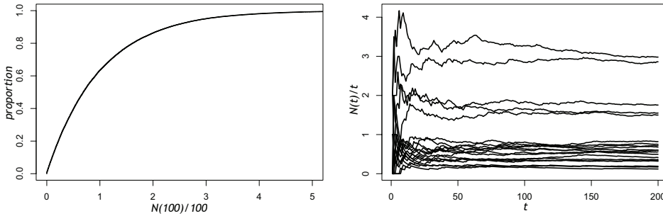
FIGURE 1: Display of the empirical distribution of N(100)/100 (left) and 25 individual sample paths of N(t)/t over [0, 200] (right) for a stationary Polya point process N with (\beta, \gamma) = (1, 1) .
