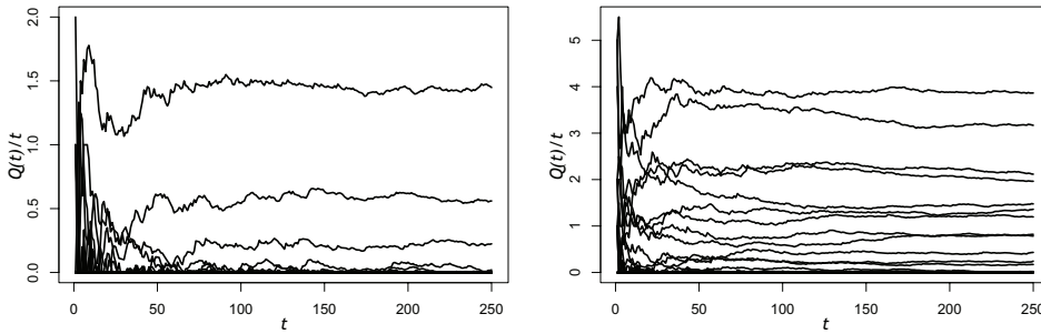
FIGURE 3: Display of twenty-five individual sample paths of Q(t)/t for 0 \leq t \leq 250 , starting empty, for a P/D/1 queue with parameter pairs (\beta, \gamma) = (0.5, 1) (left) and (\beta, \gamma) = (1.5, 1) (right).
