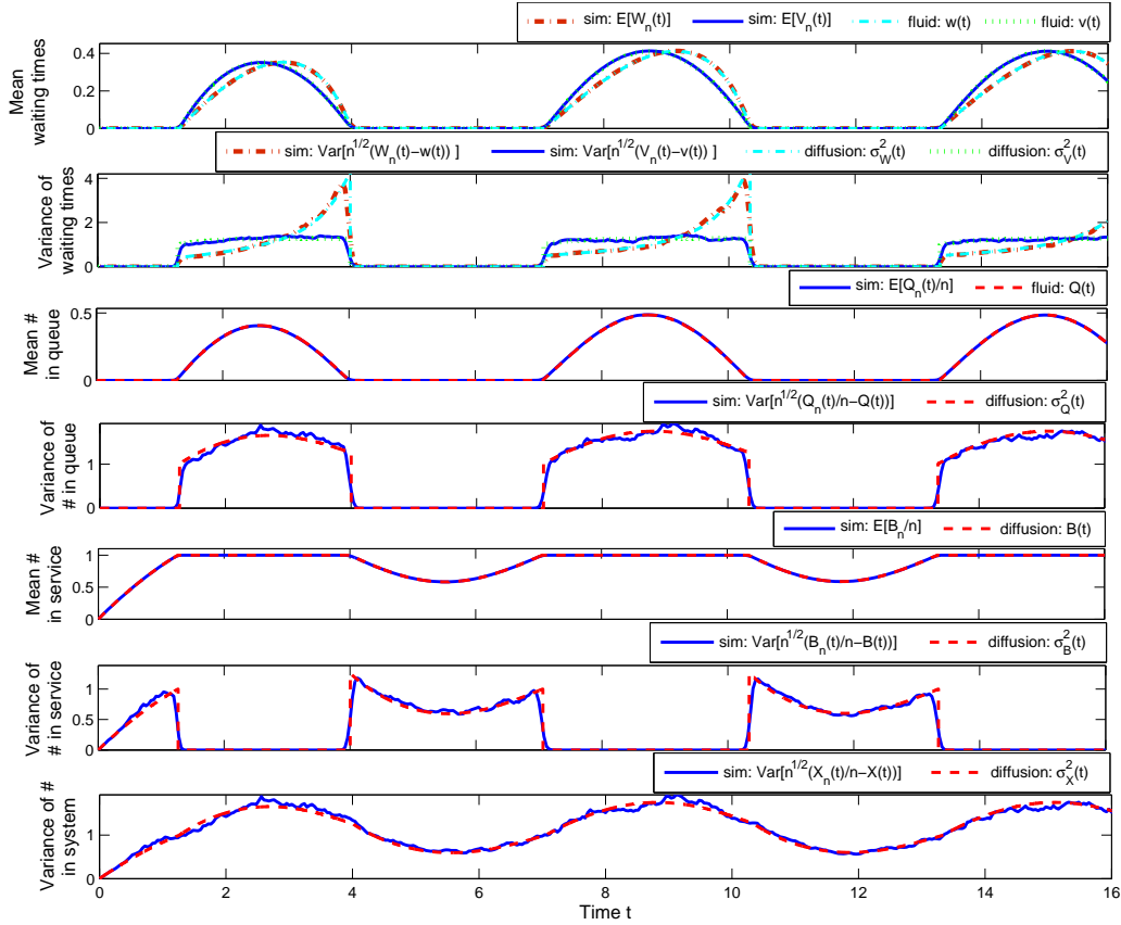
FIG 1. Comparison of the limiting means (fluid limits) and variances of the Gaussian limits to simulation estimates of the corresponding scaled queueing processes for the M_t/M/s+H_2 model starting empty for the case n = 2000 based on 500 independent replications: (i) the boundary and potential waiting times, w(t) and v(t) , (ii) the variances of the two waiting times, (iii) mean number in queue, Q(t) , (iv) the variance of the number in queue, (v) mean number in service, B(t) , (vi) variance of number in service, and (vii) variance of the total number in the system, X(t) .
