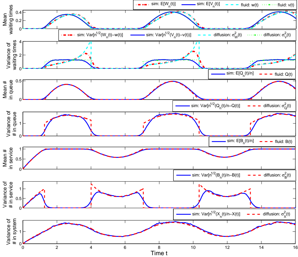
FIG 2. Comparison of the limiting means (fluid limits) and variances of the Gaussian limits to simulation estimates of the corresponding scaled queueing processes for the M_t/M/s+H_2 model starting empty for the case n = 100 based on 2000 independent replications: (i) the boundary and potential waiting times, w(t) and v(t) , (ii) the variances of the two waiting times, (iii) mean number in queue, Q(t) , (iv) the variance of the number in queue, (v) mean number in service, B(t) , (vi) variance of number in service, and (vii) variance of the total number in the system, X(t) .
