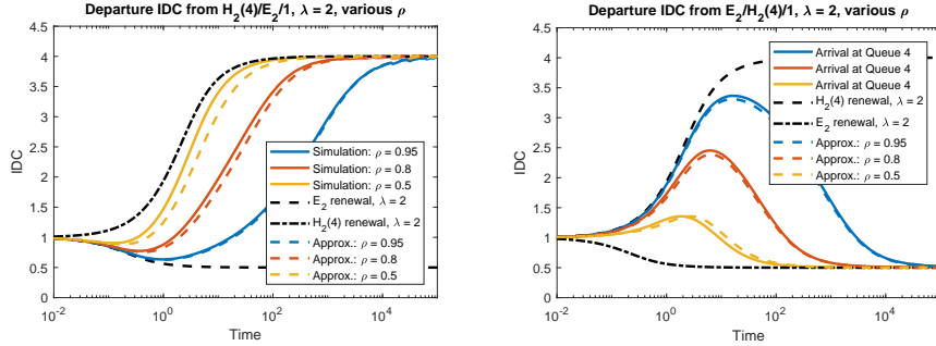
FIG 2. On the left is the IDCs of the departure from H_2(4)/E_2/1 model with \lambda = 2 and three different traffic intensities, together the two reference IDCs, one for H_2(4) and one for E_2 , displayed in broken black lines. The approximation (6.7) and (6.8) are displayed in broken colored lines. On the right is a similar plot for the E_2/H_2(4)/1 model.
