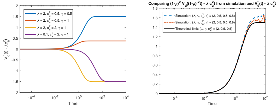
FIG 1. On the left is V^*(t) - \lambda c_a^2 t for four sets of parameters calculated from numerically inverting (3.12). On the right is the the HT-scaled variance (1 - \rho)^2 V((1 - \rho)^{-2}t) - \lambda c_a^2 t for \rho = 0.8 and 0.9 in the E_2/M/1 model, estimated by simulation, compared with the theoretical limit V^*(t) - \lambda c_a^2 t .
