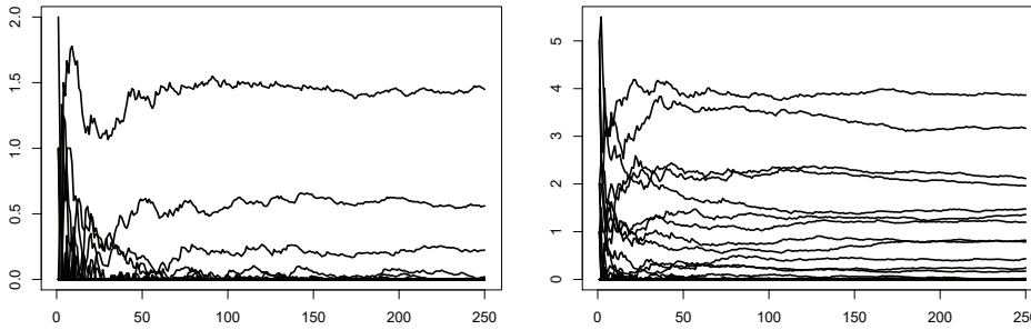
FIGURE 2: Display of twenty-five individual sample paths of Q(t)/t over [0, 250] for a P/D/1 queue with (\beta, \gamma) = (1, 1) .
