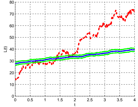
Figure 9: Linear arrival rate and H_2 service with QoS parameter \beta = 1 - L(t) of a sample path (dashed line) with an extreme value of W_{L,\lambda,q,p}(t) on [0, 4] . Average L(t) with associated 95% confidence interval based on 100 replications are also shown.
