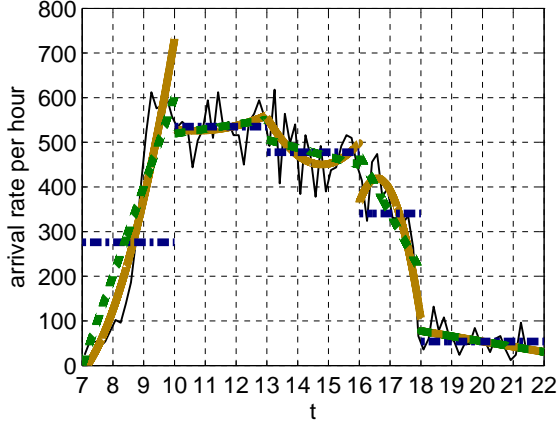
Figure 12: Arrival rate and its approximations by constant, linear and quadratic functions fitted to 5 intervals, [7, 10] , [10, 13] , [13, 16] , [16, 18] and [18, 22] , on May 7.
