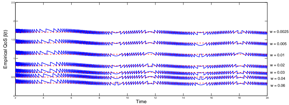
Figure 4: The empirical Quality of Service (QoS) provided by the DIS-MOL staffing in the (M_t(0.2)/\{H_2(1, 4), H_2(5, 4)\}/s_t + \{M(2), M(1)\}) + (0.2, H_2(1, 4)/\infty) example of Figure 3 as a function of the waiting-time target w .
