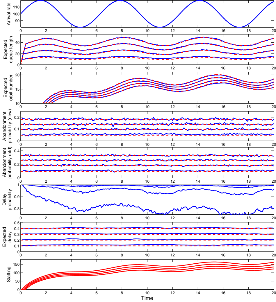
Figure 2: Performance functions in the (M_t(0.2)/\{H_2(1,4), H_2(5,4)\}/s_t + \{M(2), M(1)\}) + (0.2, H_2(1,4)/\infty) model with the sinusoidal arrival rate in (19) for \bar{\lambda} = 100 and r = 0.2 , Bernoulli feedback with probability p = 0.2 and an IS orbit queue: four cases of high waiting-time (low QoS) targets ( w = 0.10, 0.20, 0.30 and 0.40 ) and simple DIS staffing.
