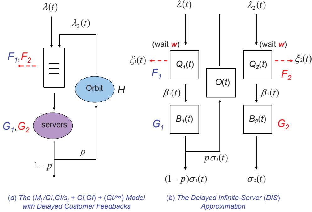
Figure 1: The (M_t / \{GI, GI\} / s_t + \{GI, GI\}) + (GI / \infty) model with delayed customer feedback and its Delayed Infinite-Server (DIS) approximation. The approximating offered load is m(t) = m_1(t) + m_2(t) \equiv E[B_1(t)] + E[B_2(t)] .
