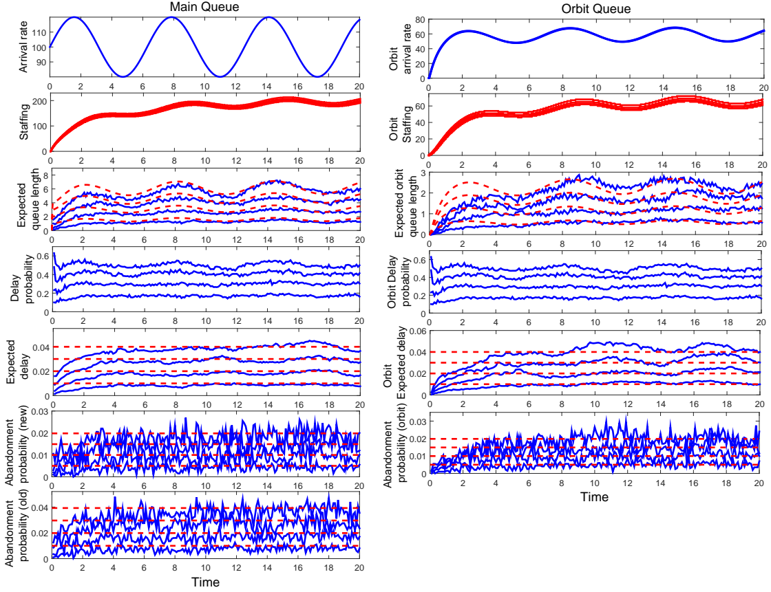
Figure 8: Performance functions in the (M_t(0.2)/\{H_2(1,4), H_2(10/6,4)\}/s_t + \{M(2), M(1)\}) + (0.6, H_2(1,4)/s_t + M(1)) model with the sinusoidal arrival rate in (19) for \bar{\lambda} = 100 and r = 0.2 , Bernoulli feedback with probability p = 0.6 and an IS orbit queue: four cases of low waiting-time (high QoS) targets ( w = 0.01, 0.02, 0.03 and 0.04 ) and DIS-MOL staffing.
