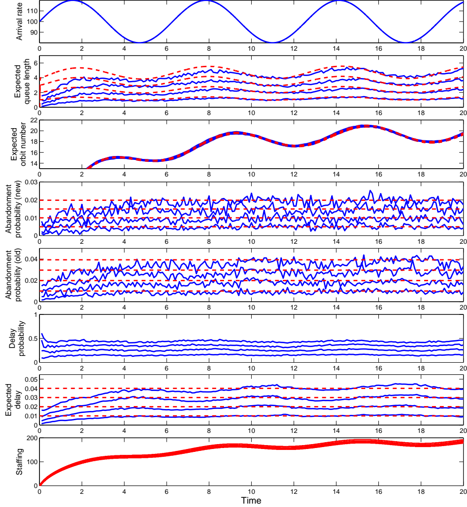
Figure 3: Performance functions in the (M_t(0.2)/\{H_2(1,4), H_2(5,4)\}/s_t + \{M(2), M(1)\}) + (0.2, H_2(1,4)/\infty) model with the sinusoidal arrival rate in (19) for \bar{\lambda} = 100 and r = 0.2 , Bernoulli feedback with probability p = 0.2 and an IS orbit queue: four cases of low waiting-time (high QoS) targets ( w = 0.01, 0.02, 0.03 and 0.04 ) and DIS-MOL staffing.
