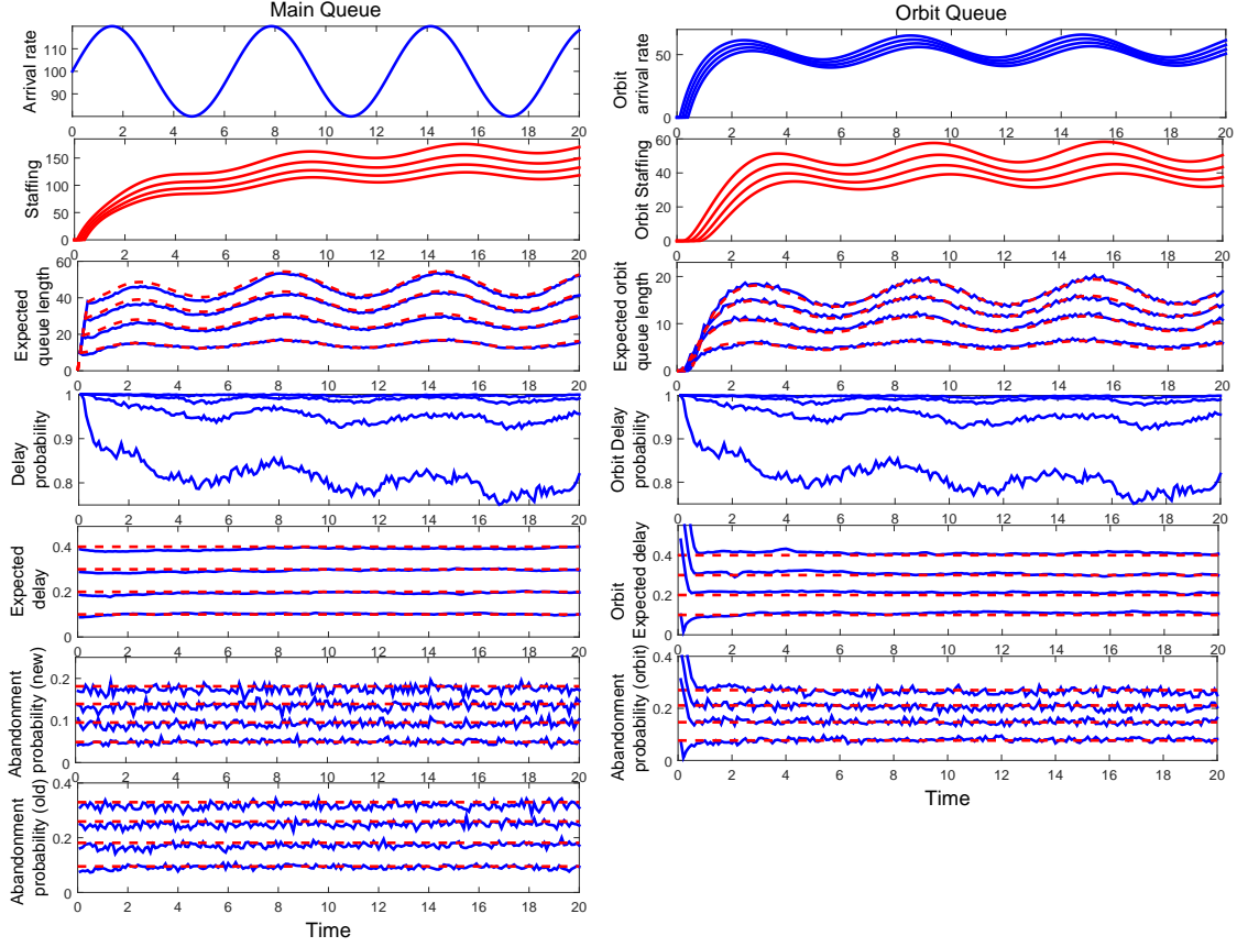
Figure 7: Performance functions in the (M_t(0.2)/\{H_2(1,4), H_2(10/6,4)\}/s_t + \{M(2), M(1)\}) + (0.6, H_2(1,4)/s_t + M(1)) model with the sinusoidal arrival rate in (19) for \bar{\lambda} = 100 and r = 0.2 , Bernoulli feedback with probability p = 0.6 and a finite-capacity orbit queue: four cases of identical high waiting-time (low QoS) targets ( w = 0.10, 0.20, 0.30 and 0.40 ) and simple DIS staffing at both queues.
