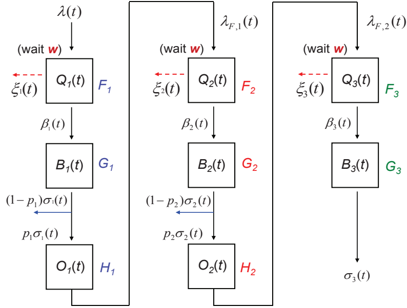
Figure 9: The DIS approximation for the (M_t/\{GI, GI, GI\}/s_t + \{GI, GI, GI\}) + (GI/\infty) + (GI/\infty) model with two delayed customer feedback opportunities. Here there are two IS orbit queues. The approximating offered load is m(t) = m_1(t) + m_2(t) + m_3(t) \equiv E[B_1(t)] + E[B_2(t)] + E[B_3(t)] .
