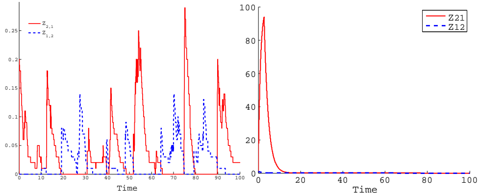
FIG 14. simulated sample path of (Z_{1,2}^n, Z_{2,1}^n) when \mathcal{O} = \phi ; n = 100 , \lambda^n = 98 , \mu = 0.5 , \theta = 0.5 , \tau^n = 1 and k_{i,j}^n = 10
