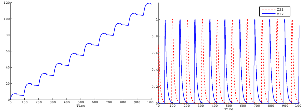
FIG 6. trajectory of q_1 increases in oscillatory manner; \theta = 0 , \mu = 0.1 .
