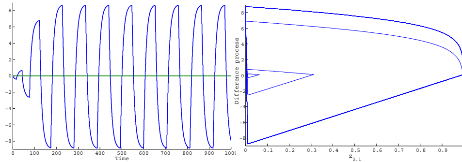
FIG 4. increasing oscillations of the difference process \Delta towards the periodic equilibrium, with \Delta(0) = 0.2 > \kappa , \theta = 0 and \mu = 0.1 .
