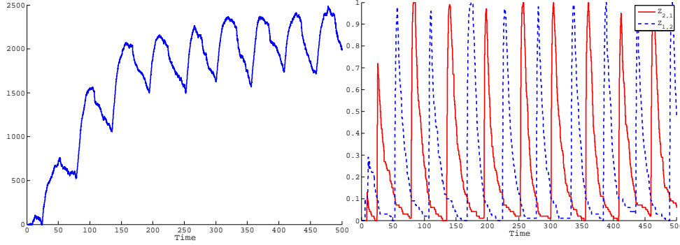
FIG 12. simulated sample path of Q_1^n ; n = 100 , \lambda^n = 98 , \kappa^n = 10 , \theta = 0.01 , \mu = 0.1
