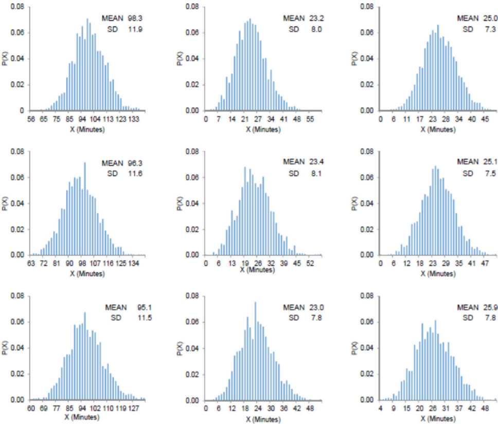
Figure 1 — A 3 × 3 collage of histograms of total waiting times for group 75 over 2000 simulation replications. Each row represents three different course designs: (i) the base case, (ii) the par-5-holes first and (iii) the par-3 holes first. Each column represents three different types of par-3 holes in the golf course: P3 , SP3 , and P2WU . In all of the nine histograms, the tee interval is 7.50 minutes.
