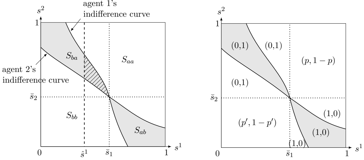
Figure 3: Bayesian Implementation
