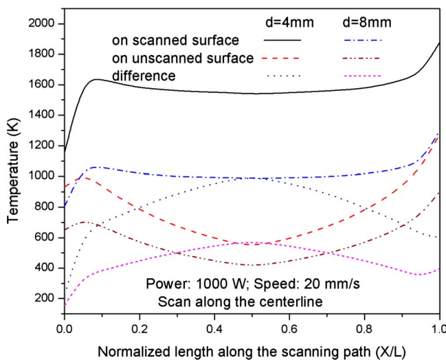
Fig. 12 Temperature distribution of varying thickness coupon under various beam spot sizes (power=1000 W, d=4 mm and 8 mm, single scan along the centerline)
