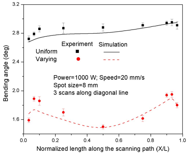
Fig. 9 Bending angle variation along the scanning path when scanned along the diagonal line
