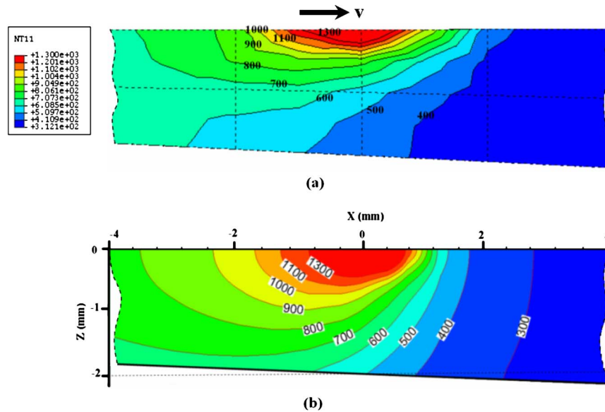
Fig. 15 Temperature field at the cross section along the scanning path of varying thickness plate (a) obtained by FEM, and (b) obtained by the analytical method (under the condition of power=1000 W, V=20 mm/s, the coordinate system refers to Fig. 1)
