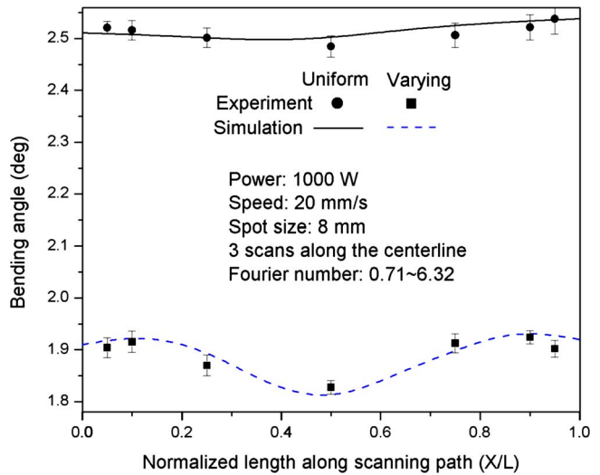
Fig. 2 Bending angle variation of varying thickness plate and uniform-thickness ( h=2 mm) plate along the scanning direction
