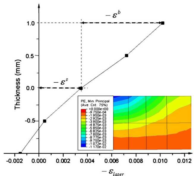
Fig. 6 Strain distribution through thickness, showing the definition of bending and in-plane strain
