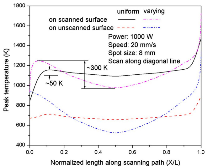
Fig. 10 Comparison of peak temperature along the scanning path between varying and equivalent-uniform thickness plate when scanned along diagonal line
