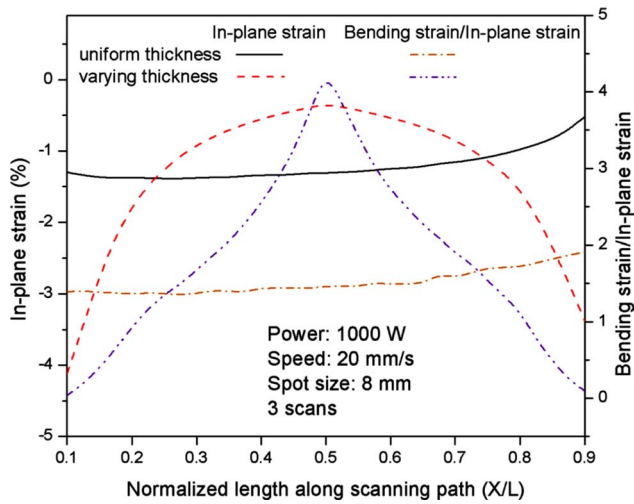
Fig. 7 Distribution of in-plane strain and ratio of bending strain to in-plane strain
