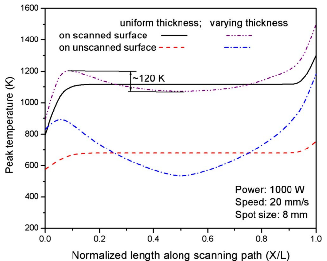
Fig. 3 Comparison of the temperature distribution along the scanning path between varying thickness plate and equivalent-uniform thickness ( h=2 mm) plate
