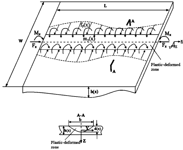
Fig. 16 Schematic of the mechanical model
