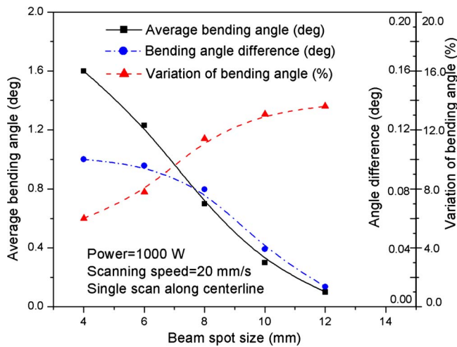
Fig. 11 Bending deformation of varying-thickness coupon under various beam spot sizes (power=1000 W, scanning speed =20 mm/s, single scan along the centerline)
