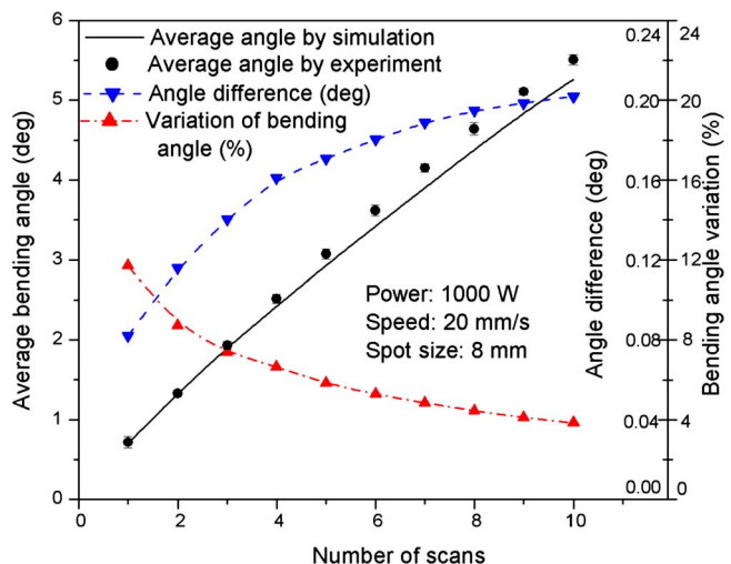
Fig. 14 The relationship between bending angle and number of scans (power=1000 W, scanning speed=20 mm/s, spot size=8 mm)
