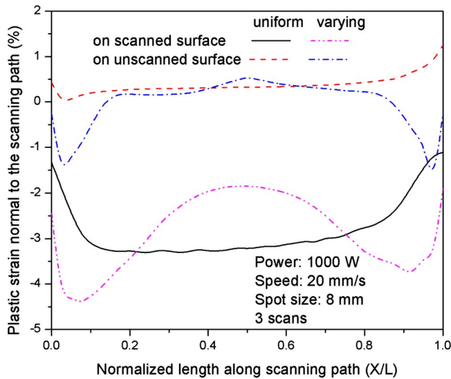
Fig. 4 Comparison of the plastic strain normal to the heating direction between varying thickness plate and equivalent-uniform thickness ( h=2 mm) plate
