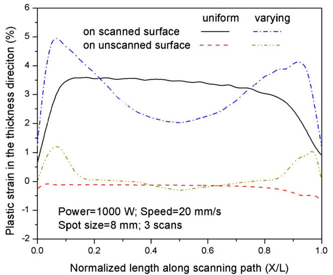
Fig. 5 The distribution of plastic strain in thickness direction along the scanning path
