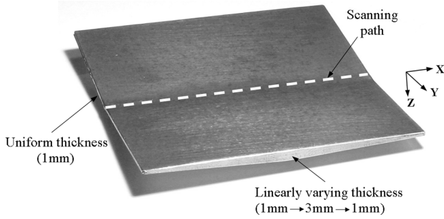
Fig. 1 Laser formed varying thickness plate showing coordinate system (scanned along the centerline, plate size: 80 × 80 mm, power=1000 W, scanning speed=20 mm/s, beam spot size=8 mm, number of scans=10)
