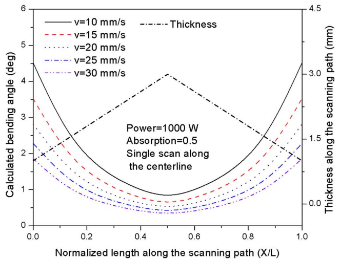
Fig. 17 Bending angle variations with thickness under different scanning speed (a) obtained by FEM, and (b) obtained by the proposed model
