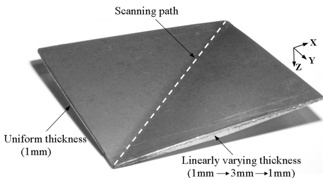
Fig. 8 Experimental result of varying thickness plate scanned along the diagonal line (plate size: 80 × 80 mm, linearly varying thickness; power=1000 w, scanning speed=20 mm/s, beam spot size=8 mm, number of scans=10)
