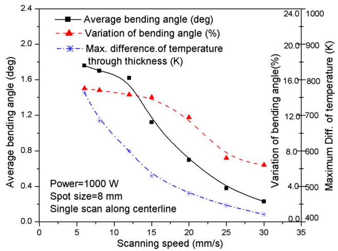
Fig. 13 Bending deformation of varying thickness coupon under various scanning speeds (power=1000 w, spot size =8 mm, single scan along the centerline)
