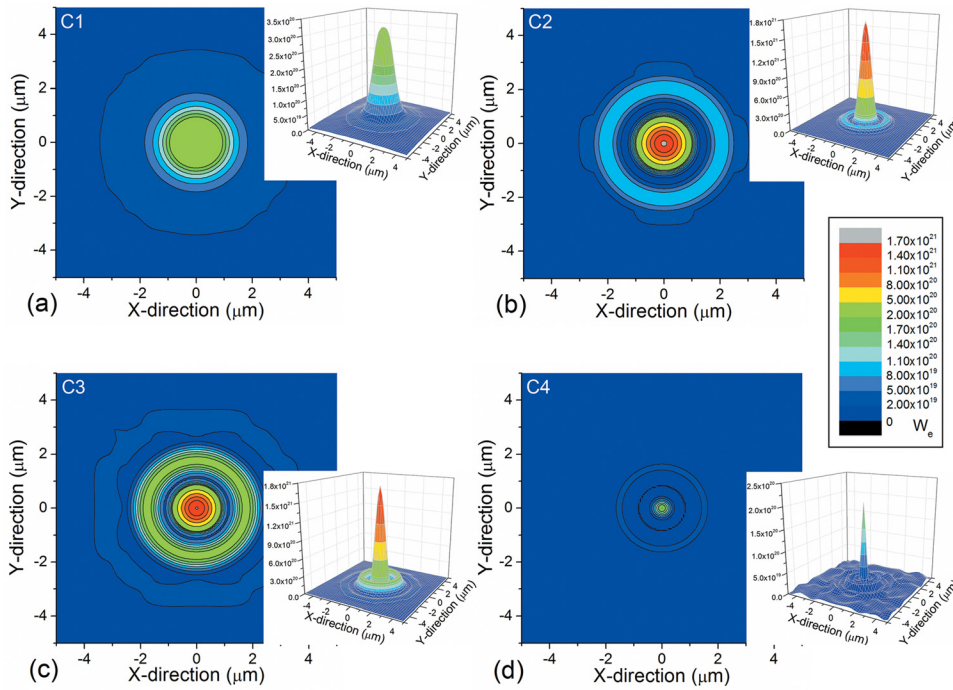
FIG. 14. The contour and 3D surface maps in xy-planes along (a) line C1 located along the paraxial-ray focal plane, (b) line C2 located along the highest peak of electric energy density, (c) line C3 located along the second highest peak of electric energy density, and (d) line C4 located along the peripheral-ray focal plane.
