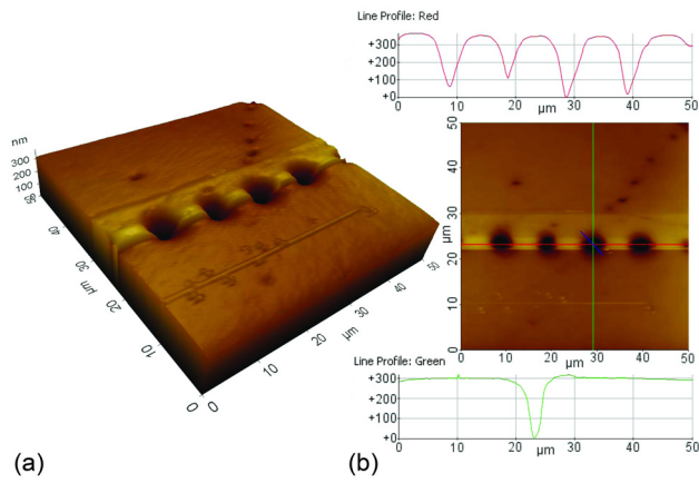
FIG. 4. (a) 3D AFM topography and (b) the AFM top view image and line profiles across the channels on the new polished surface (xy-plane) across the channels irradiated by a series of single pulse energy of 30 \mu\text{J} .
