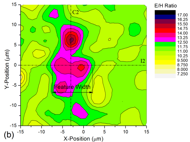
Fig. 11 Spatially resolved determination of the ratio between Young's modulus and hardness (E/H) on the cross section of (a) a welded region of two-piece specimen (b) a feature inside one-piece specimen using the same laser pulse energy of 10 μJ and scanning speed of 0.02 mm/s. The contour maps correspond to the array of 100 nm depth nanoindents with 3 μm spacing.
