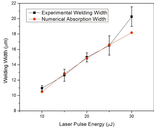
Fig. 6 Comparison of experimental weld width and simulated absorption width at different laser pulse energies. Error bars denote standard deviation.
