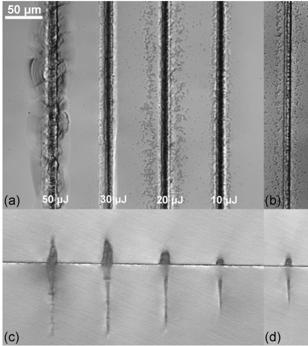
Fig. 5 (a) Top view ( xy -plane) and (c) cross section view ( xz -plane) of weld seams performed at different processing conditions obtained through transmission DIC optical microscopy (laser scanning speed of 0.06 mm/s, 0.04 mm/s, 0.03 mm/s, and 0.02 mm/s, respectively, from the left) (b) Top view ( xy -plane) and (d) cross section view ( xz -plane) of a weld seam for 10 \mu J and 0.02 mm/s condition
