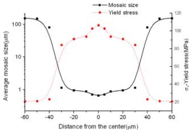
Fig. 17 Spatial distribution of average mosaic size from initial slope analysis by FFT and shock-induced strengthening effects for Al (110)
