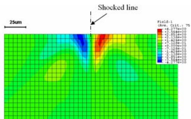
Fig. 4 Typical lattice rotation field on cross section after laser shock peening, Al (110) sample: 200 \times 100 \mu\text{m} as shown; total simulation region is 800 \times 400 \mu\text{m} .
