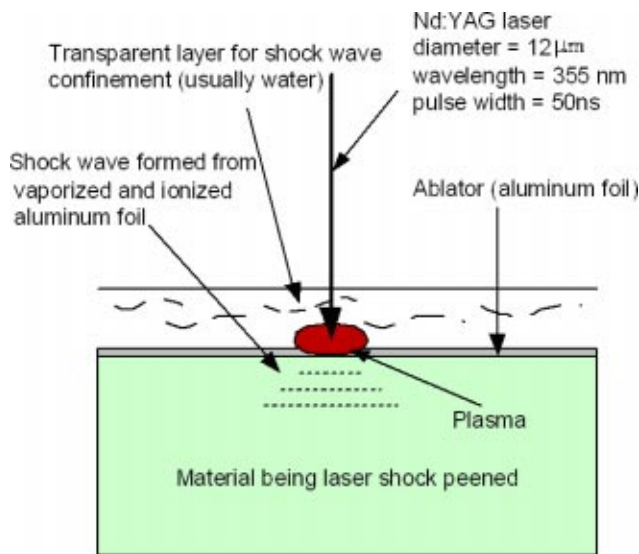
Fig. 1 Laser shock-peening process
