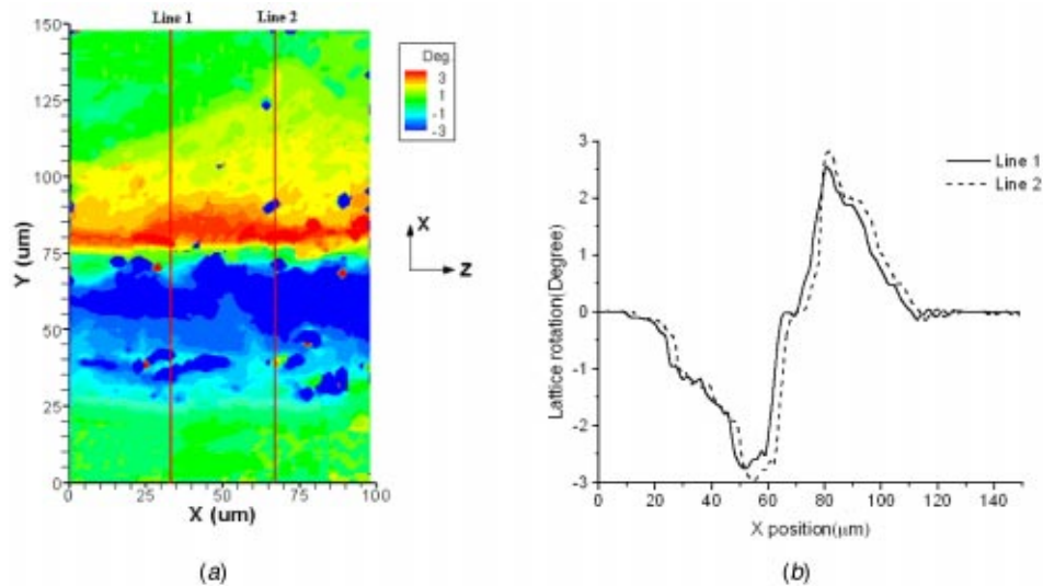
Fig. 14 Lattice rotation contour map on sample surface for Al(110) sample (line 1–2: two cross sections with spacing=34 \mu\text{m} )
