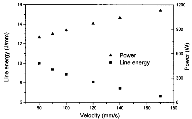
Fig. 5 Experimental values of line energy and laser power under the condition of constant peak temperature
