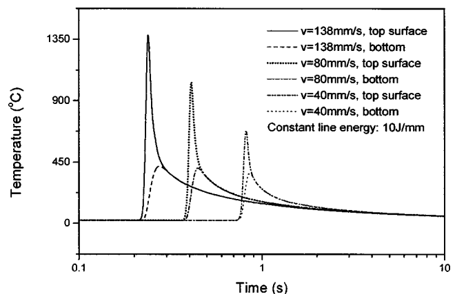
Fig. 3 Simulated time histories of temperature under the condition of constant line energy [17]
