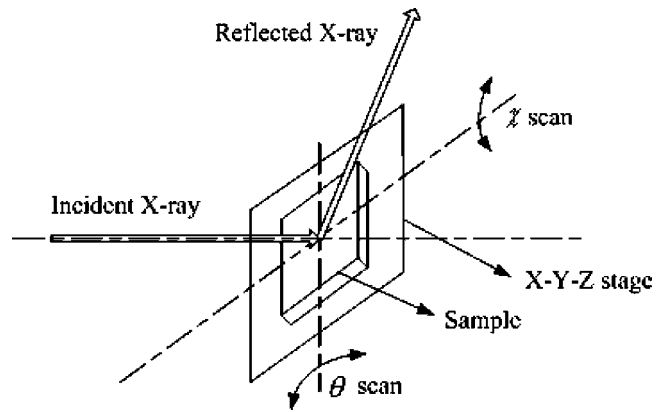
Fig. 6 \theta and \chi scan of sample/stage
