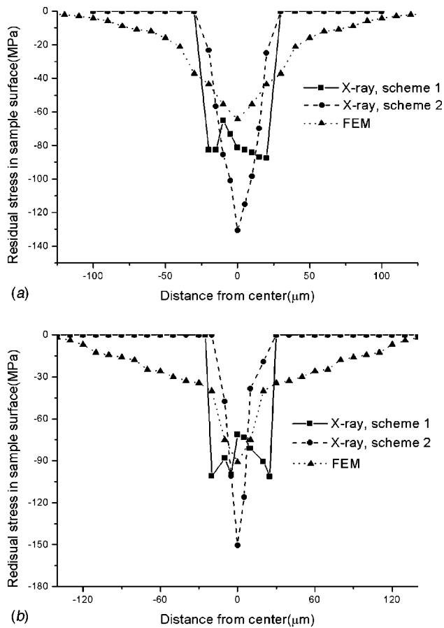
Fig. 11 Comparison of spatial residual stress distribution on sample surface by two X-ray measurement schemes and FEM simulation. (Laser beam diameter is 12 microns, pulse duration is 50ns, laser pulse energy=300 \mu J). (a) Al (110) sample (b) Cu (110) sample
