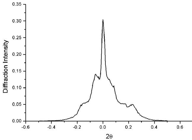
Fig. 5 Incident X-ray micro beam profile Full width at half maximum intensity (FWHM) \approx 0.05^\circ (\pm 0.025^\circ)
