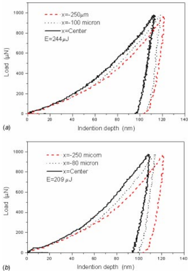
Fig. 10 Loading and unloading curves measured at different locations of shocked 1\ \mu\text{m} samples (a) 244\ \mu\text{J} and (b) 209\ \mu\text{J} . The dashed line, measured far away (250 microns) from the shock center, represents the reference curve.
