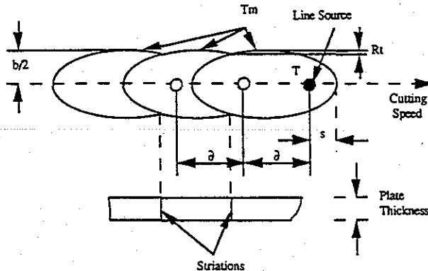
Figure 1. Conceptual model for stria formation
