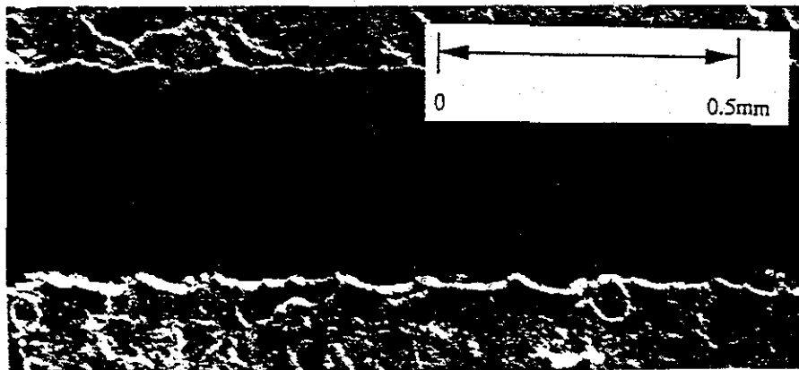
Figure 5. The edge profile observed in specimen 9
