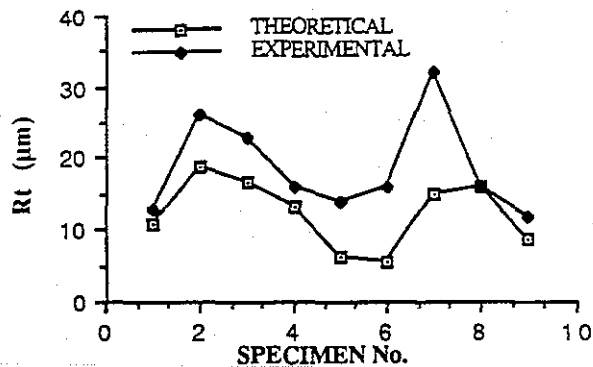
Figure 6. R_t values for each specimen
