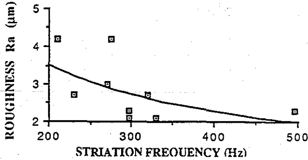
Figure 2. Correlation between surface roughness and striation frequency
