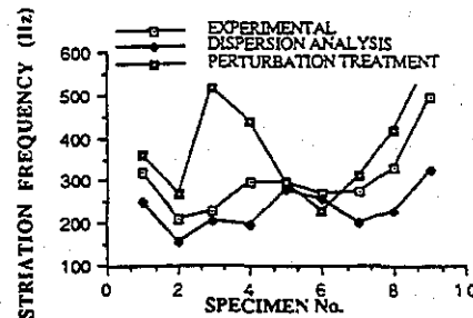
Figure 4. Striation frequencies for each specimen
