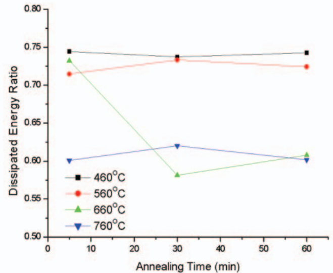
FIGURE 9: DISSIPATED ENERGY RATIO VS ANNEALING TIME AT VARIOUS TEMPERATURES. NOTE REDUCED DISSIPATION FOR HIGHER TEMPERATURE HEAT TREATMENTS DUE TO AUSTENITIC STRUCTURE
