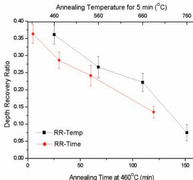
FIGURE 11: RECOVERY RATIO AS A FUNCTION OF ANNEALING TEMPERATURE AND TIME. ERROR BARS DENOTE STANDARD ERROR
