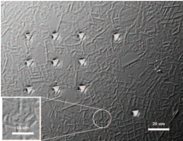
FIGURE 6: OPTICAL MICROGRAPH OF RESIDUAL IMPRESSIONS FROM 1 \mu m AND 100nm (INSET) DEEP INDENTATIONS ON ANNEALED NiTi FILM BEFORE HEATING. FILM ANNEALED AT 460°C FOR 5 MINUTES
