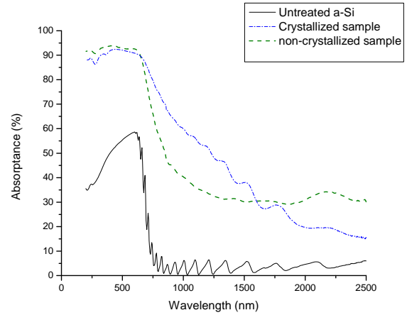
Figure 11. Comparison of absorbance spectra of a-Si:H films with and without crystallinity at different fluences and scanning speeds (0.5J/cm 2 at 25mm/s, 1.2J/cm 2 at 2mm/s) in water, showing the effect of crystallinity on absorption
