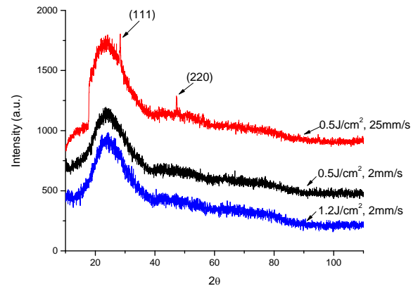
Figure 9. X-ray diffraction spectra of a-Si:H films laser treated at fluences of 0.5\text{J/cm}^2 and 1.2\text{J/cm}^2 , and scan speeds of 2mm/s and 25 mm/s in water. An “amorphous peak” around 2\theta=25^\circ is observed for all samples. Sample processed at 0.5\text{J/cm}^2 and 25mm/s shows existence of two peaks for (111) and (220) orientation of silicon, showing the effect of different laser parameters on crystallinity
