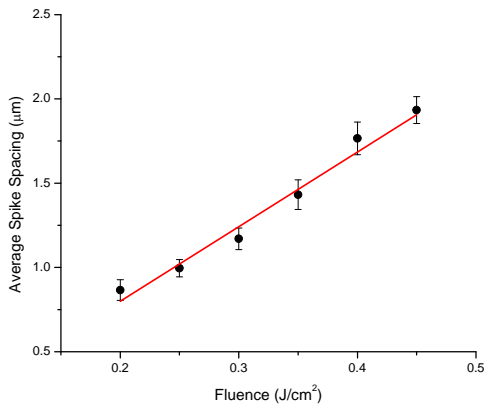
Figure 3. Dependence of average spike spacing on laser fluence for a fixed number of pulses (100 pulses) after treated in air, determined from an area of 50 \times 50 \mu\text{m}^2 at the processing center, error bars indicate standard deviation.
