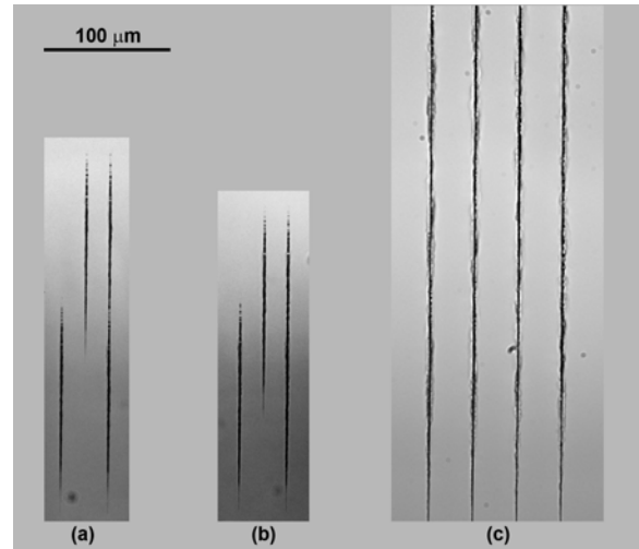
Figure 8. Cascading of two single pulses with (a) an inadequate overlapping distance, and (b) an appropriate overlapping distance. (c) Cascading of multiple single pulses using pulse energy of 30 \mu\text{J} . The above three figures have been adjusted to the same scale.
