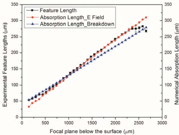
Figure 14. Comparison of feature lengths from two numerical models and experimental results at different focusing depths using laser pulse energy of 30 \mu\text{J} .
