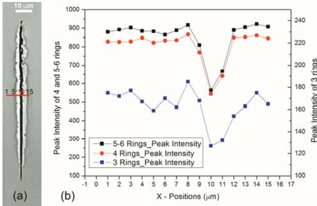
Figure 4. (a) Raman signal measurements points across the cross section view (xz-plane) of a feature and channel, and (b) the peak intensity of the 3 rings, 4 rings, and 5-6 rings structure of fifteen points across the channel.
