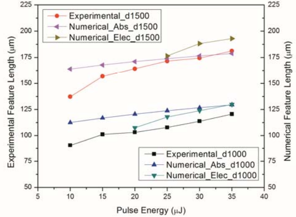
Figure 15. Comparison of feature lengths from two numerical models and experimental results at different pulse energies for focusing depth of 1000 \mu\text{m} and 1500 \mu\text{m} below the top surface of fused silica sample, respectively.
