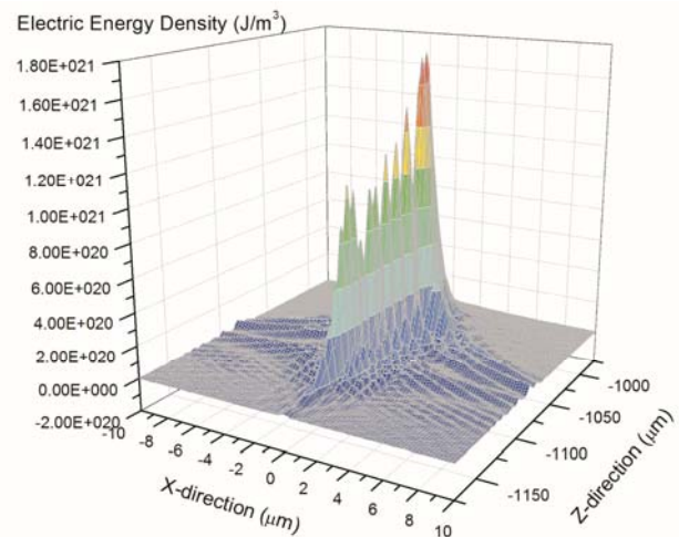
Figure 10. The 3D surface map of representative electric energy density field on the xz-plane along an optical axis in the vicinity of the focal plane for laser pulse energy of 30 \mu\text{J} at the focusing depth of 1000 \mu\text{m} .
