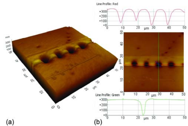
Figure 3. (a) 3D AFM topography and (b) the AFM top view image and line profiles across the channels on the new polished surface (xy-plane) across the channels irradiated by a series of single pulse energy of 30 μJ.
