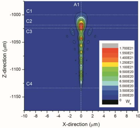
Figure 11. The contour map of representative electric energy density field on the xz-plane along an optical axis in the vicinity of the focal plane for laser pulse energy of 30 \mu\text{J} at the focusing depth of 1000 \mu\text{m} . Lines C1, C2, C3, C4, and A1 represent section lines across this field.
