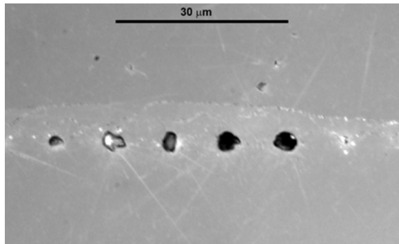
Figure 2. Refractive DIC optical microscopy of top view (xy-plane) of the new polished surface across the channels irradiated by a series of single pulse energy of 30 μJ.
