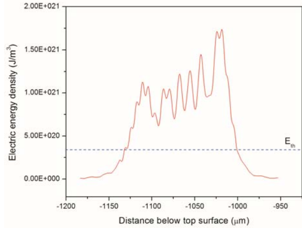
Figure 13. The electric energy density on the optical axis along line A1 in Fig. 11 compared to the damage threshold of fused silica sample.
