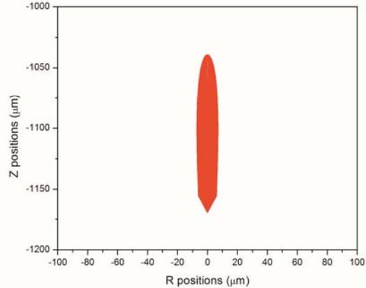
Figure 9. The representative simulated cross section (rz-plane) of the absorption volume by 30 \mu\text{J} pulse energy at the focusing depth of 1000 \mu\text{m} from the absorption volume model.
