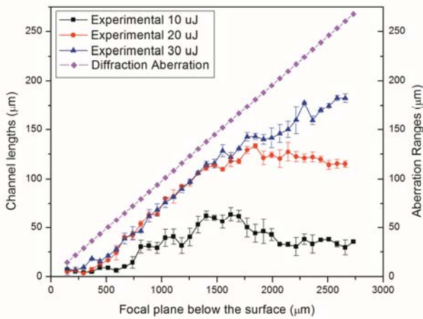
Figure 7. Comparison of experimental channel lengths at 10 \mu\text{J} , 20 \mu\text{J} , and 30 \mu\text{J} , and the diffraction limited aberration range at different focusing depths. Error bars denote standard deviation.
