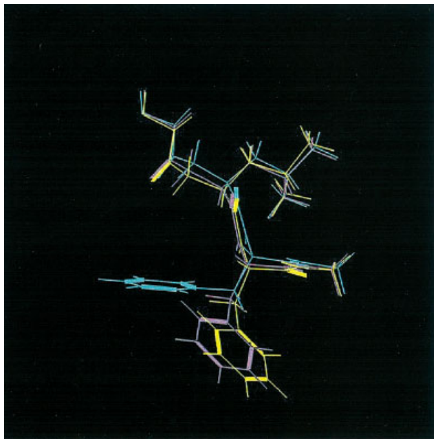
Figure 7. Overlap of native (yellow), third (green), and fourth (purple) QM Dock structures of 1hfc from Table 8.
