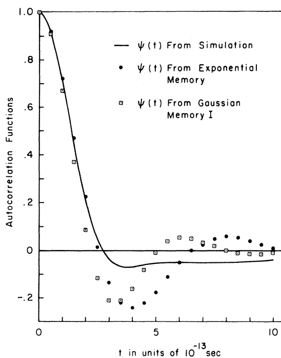
FIG. 12. Approximate velocity autocorrelation functions from the modified Stockmayer simulation using the exponential and Gaussian I memories.
