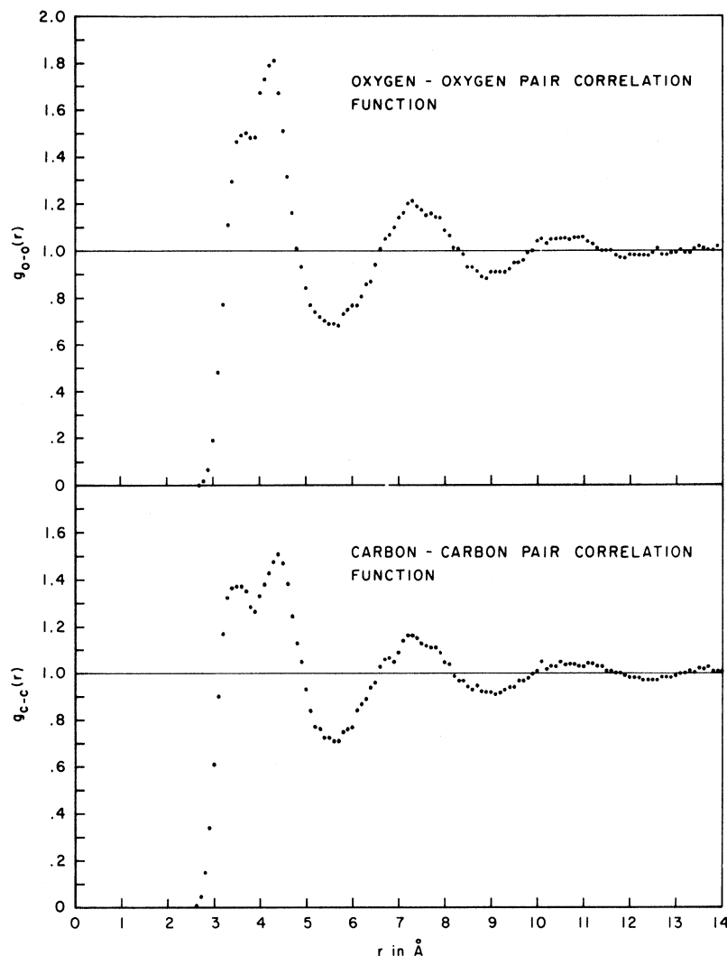
FIG. 19. The oxygen-oxygen and carbon-carbon pair-correlation function from the modified Stockmayer simulation.
