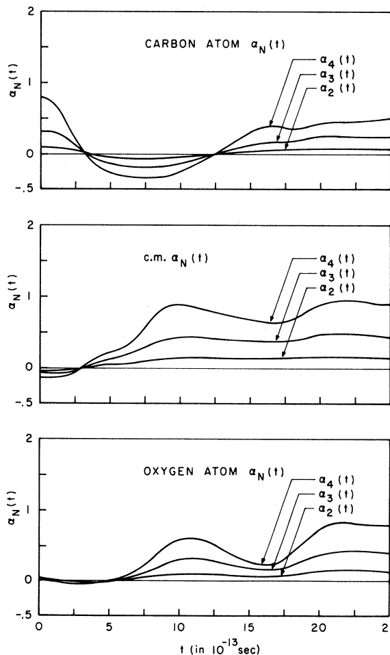
FIG. 25. Non-Gaussian behavior of G_s^{(v)}(r, t) in the Stockmayer simulation using 512 molecules.
