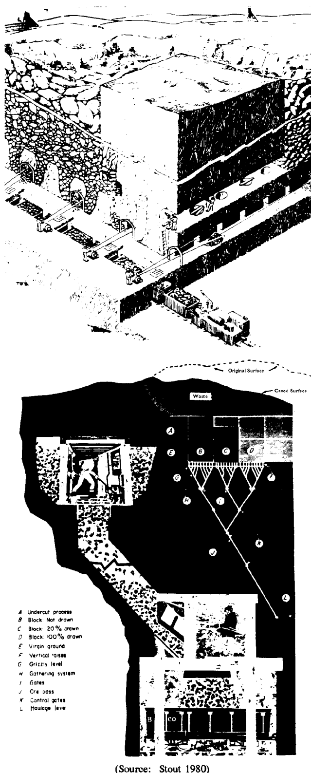
Figure 1-3. Block-Caving Methods
