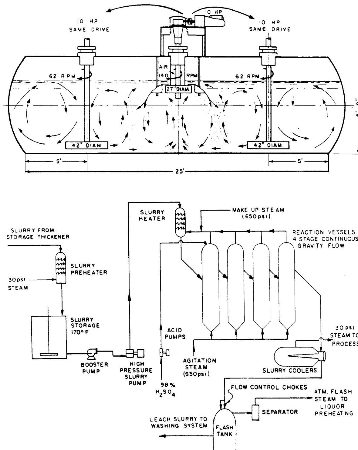
Figure 1-14. Typical Autoclave and Vat Leaching Circuit
