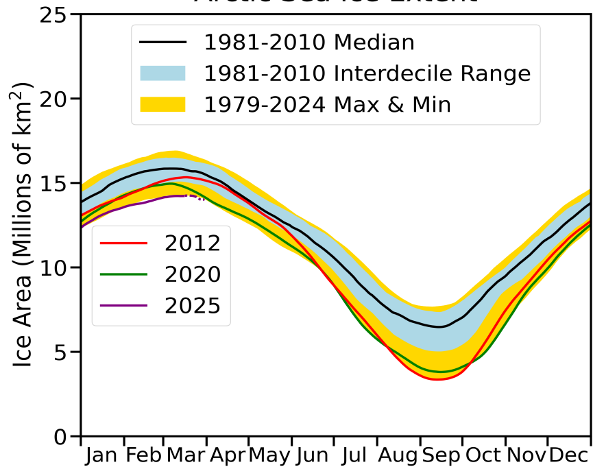
Arctic Sea Ice Extent
