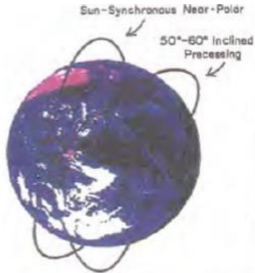
Fig. 33.1. Climsat orbits.
