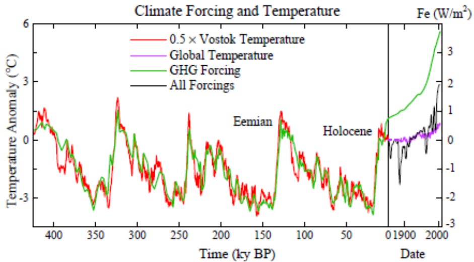
Fig. 40.2. Temperature (left scale) and climate forcing (right scale).
