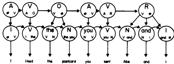
Figure 1. Two-level context-sensitive coding of the syntactic structure of the title sentence in terms of overlapping triples of syntactic class concepts. Note that the substantive noun (N), verb (V), adjective and adverb classes are assumed to be rather large classes, while the grammatical word classes—articles, pronouns, prepositions, and conjunctions—are assumed to be very small and specific classes. The lower level of syntactic coding is concerned with word classes, while the higher level is concerned with the semantic function of concepts in propositions.
