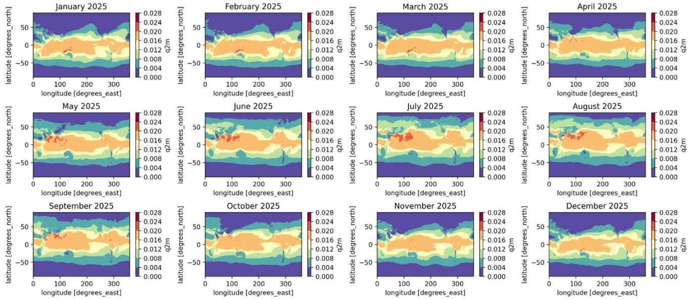
Monthly Mean Values of Specific Humidity in 2025
